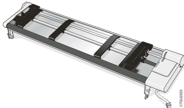
Figure 26. Second tractor
