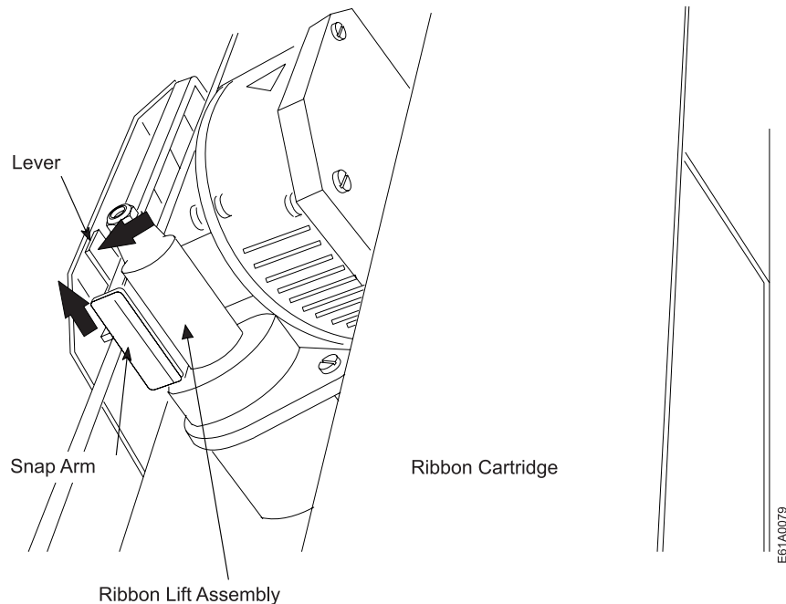
Figure 39. Freeing the shifter holder
