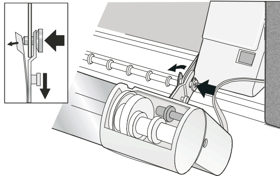
Figure 32. Disconnecting the second tractor.
