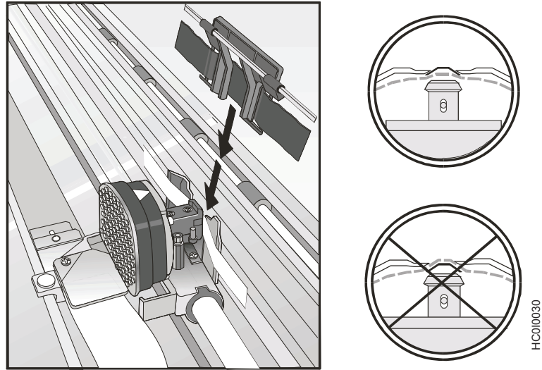
Figure 12. Print head and ribbon guide mask showing correct positioning of the ribbon.
