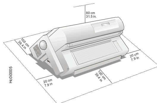
Figure 4. Printer clearances.
