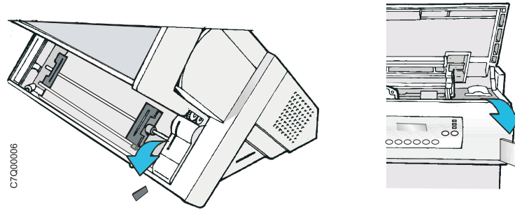
Figure 3. Removing the shipping locks from the printer.
