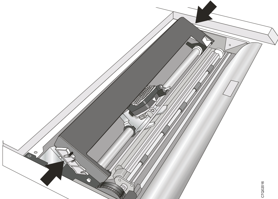
Figure 11. Aligning the cartridge pins.
