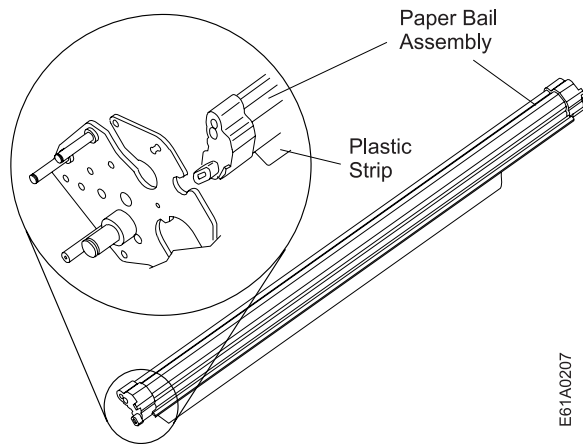
Figure 42. Inserting the left and right paper bail end cap pivots into the side frames
