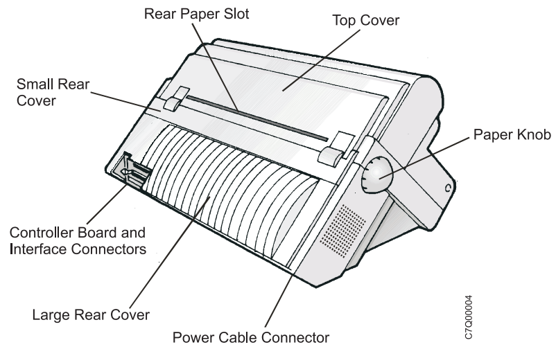
Figure 1. Printer Parts: Front and Rear View
