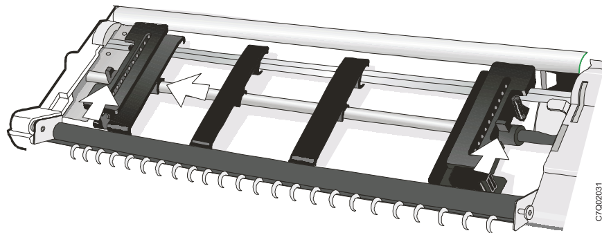
Figure 18. Unlocking the sprockets of the Front1 push tractor
