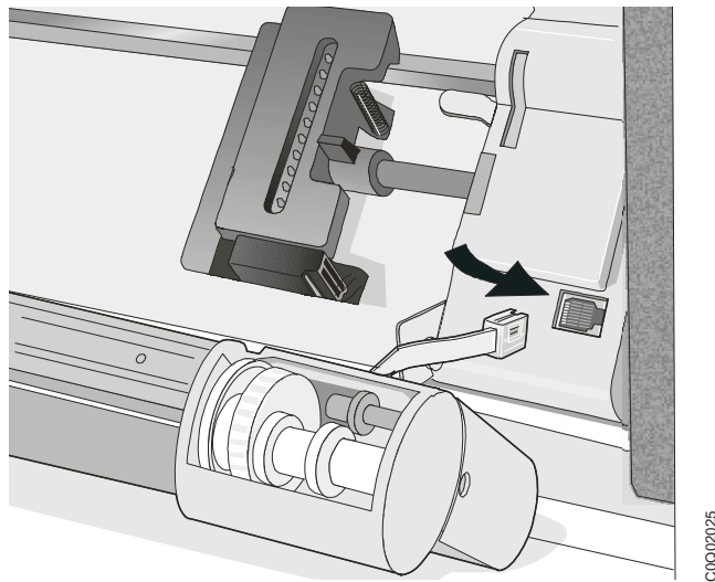
Figure 28. Connecting the second tractor
