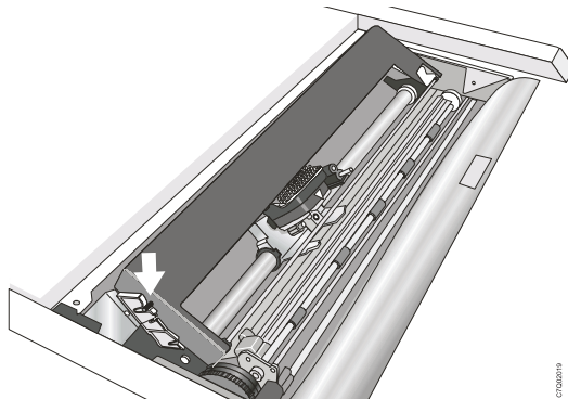
Figure 14. Aligning the ribbon mounting pins.
