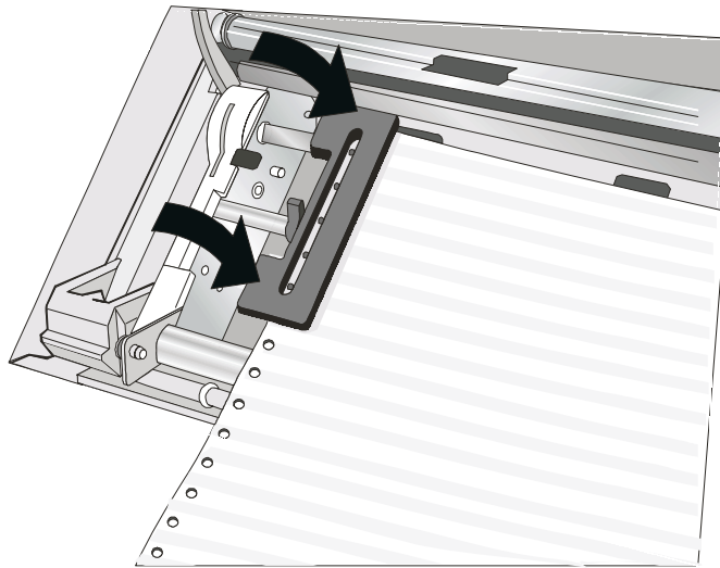
Figure 20. Closing the left sprocket cover.
