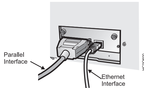
Controller Board with parallel interface and ASCII-IPDS Ethernet 10/100 LAN interface.
