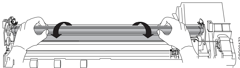
Figure 40. Rotating the bail assembly
