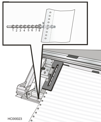
Figure 22. Matching the left sprocket for the first printing position.
