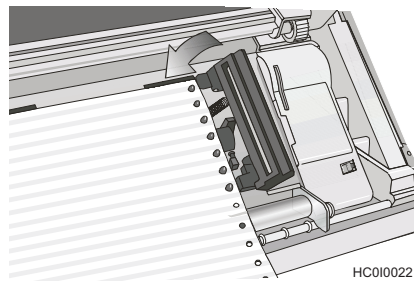
Figure 21. Inserting the paper on the right sprocket pins.
