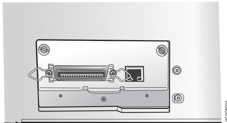
Figure 7. Attaching the Controller Board.
