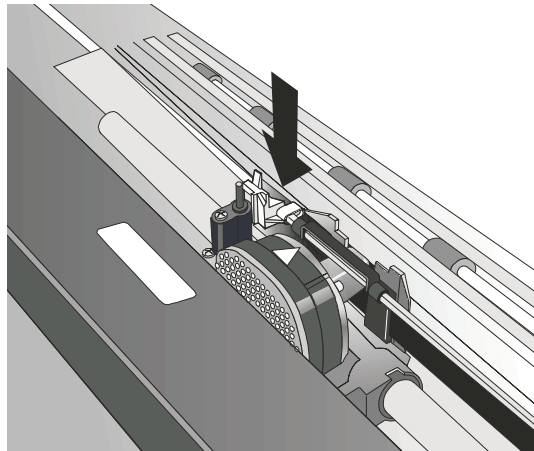
Figure 13. Positioning the snap arm.
