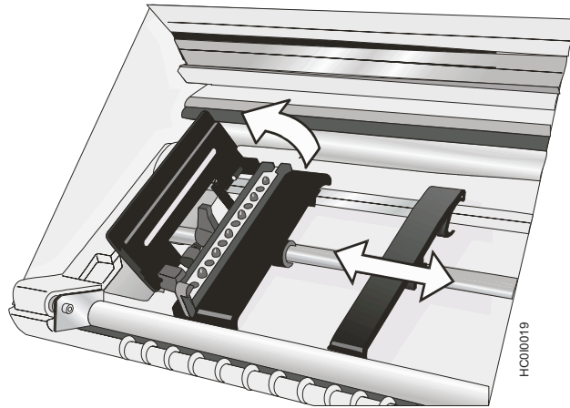
Figure 19. Opening the left and right sprocket covers.
