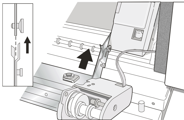
Figure 27. Aligning the second tractor hooks.
