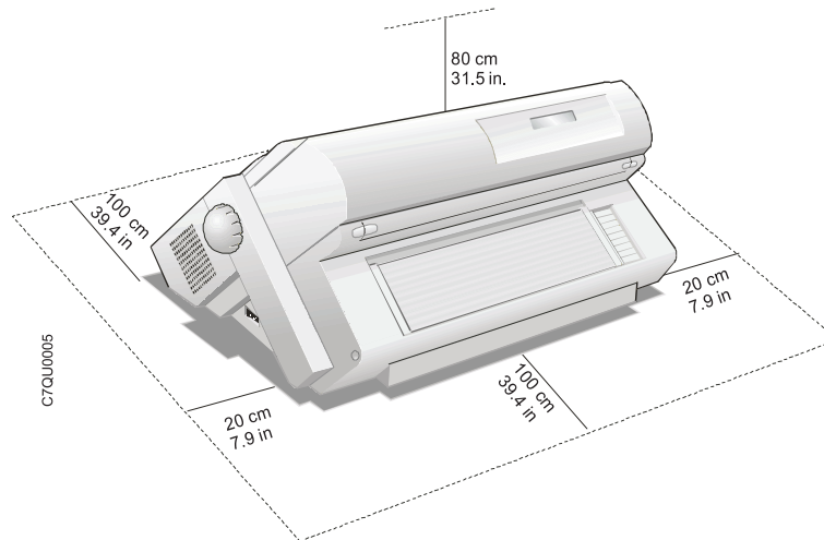
Figure 43. Printer clearances.
