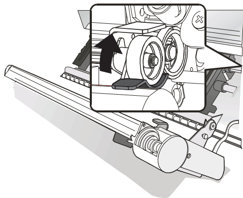
Figure 33. Closing the protection cover.
