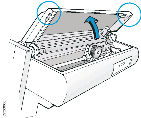
Figure 10. Opening the top cover
