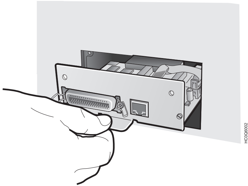
Figure 6. Sliding the board in the slot.
