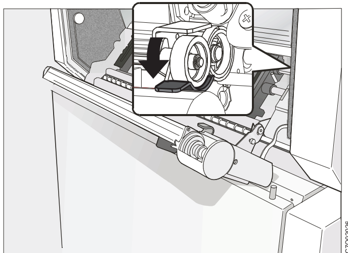
Figure 29. Rotating the tractor gear protection cover.
